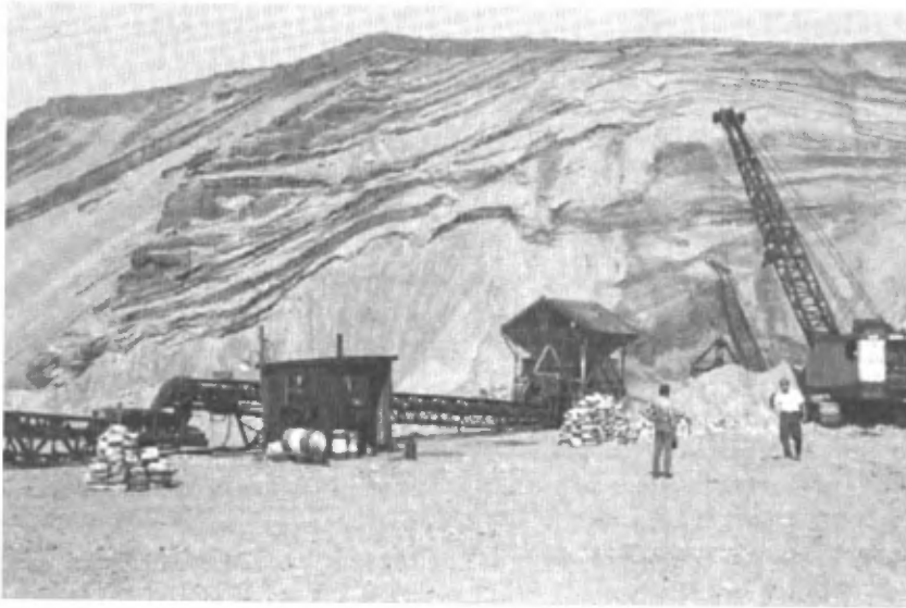
FIGURE 17 - Coupe du delta glacio-marin exploité par la compagnie Francon à Saint-Gabriel. Vue du sud-est. Gravel pit in the glacio-marine delta at Saint-Gabriel. Owned by Francon company. View from the southeast. For description, see Figure 18.
