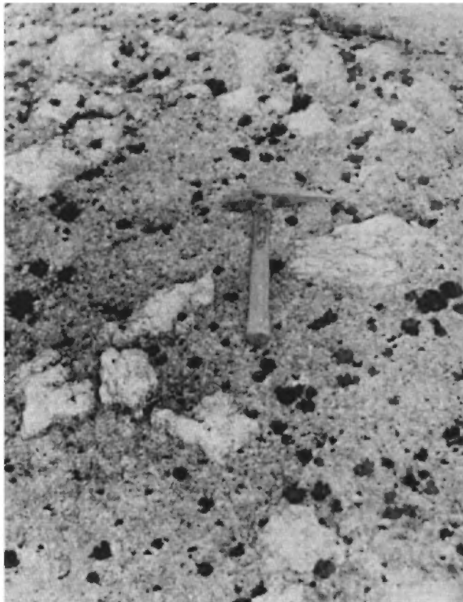
Pl. VII - Pegmatite de type "Football" "Football" pegmatite.
