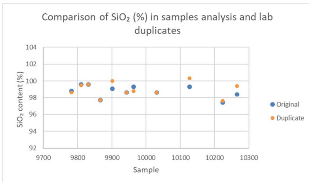
Figure 13. Comparison of \text{SiO}_2 (%) in samples analysis and lab duplicates
