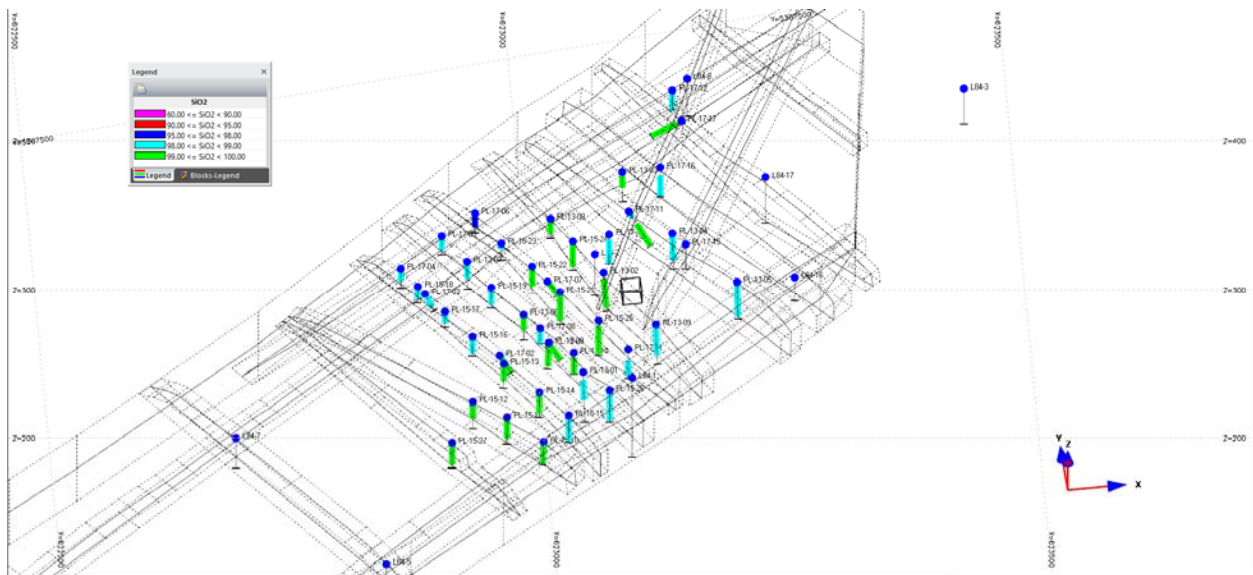
Figure 20: Perspective view of the prims and drill hole with colour coded mineralized intervals
