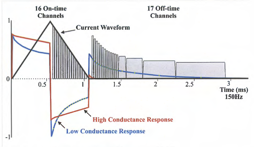
Figure 8. Schematic of Transmitter and Receiver waveforms
