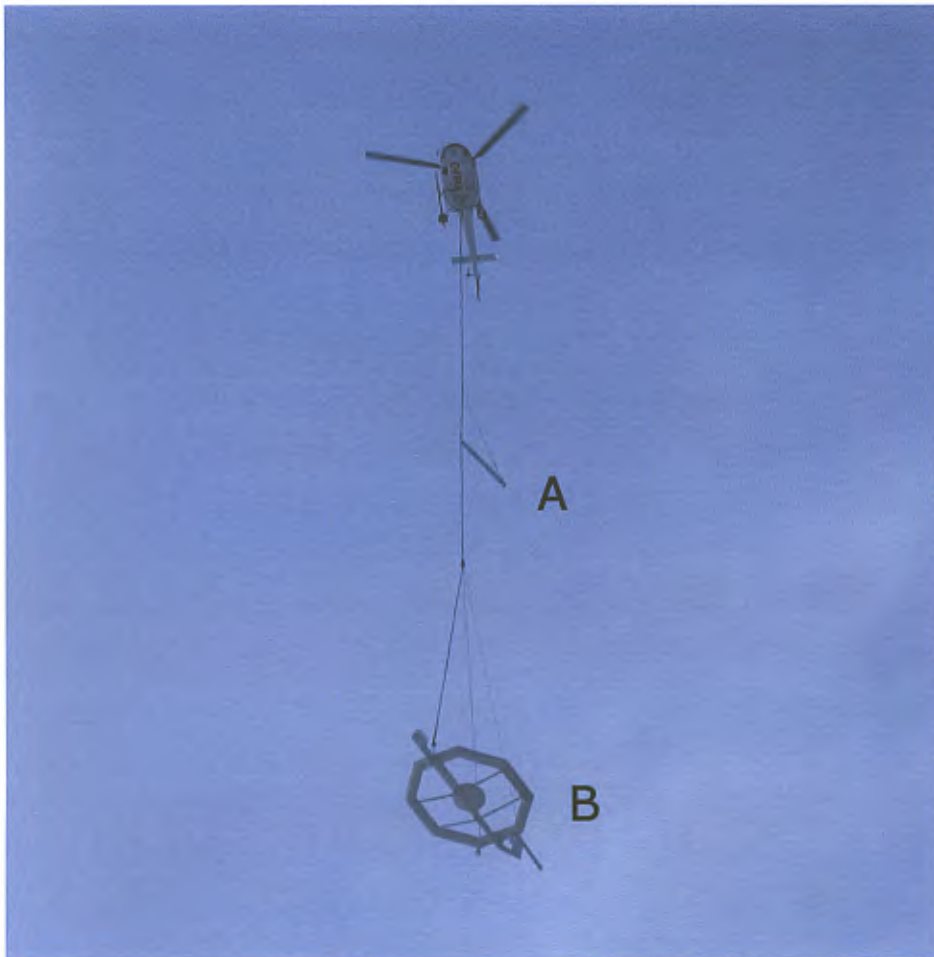
Figure 7. The magnetometer bird (A) and AeroTEM II EM bird (B)
