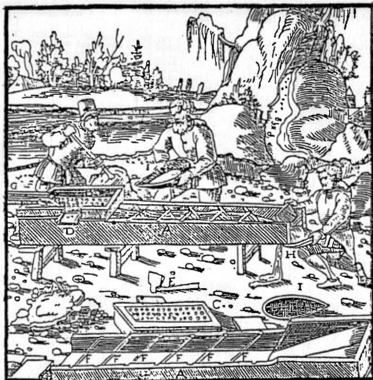
A—SLUICE. B—BOX. C—BOTTOM OF INVERTED BOX. D—OPEN PART OF IT. E—IRON HOE. F—RIFFLES. G—SMALL LAUNDER. H—BOWL WITH WHICH SETTLEMENTS ARE TAKEN AWAY. I—BLACK BOWL IN WHICH THEY ARE WASHED.
