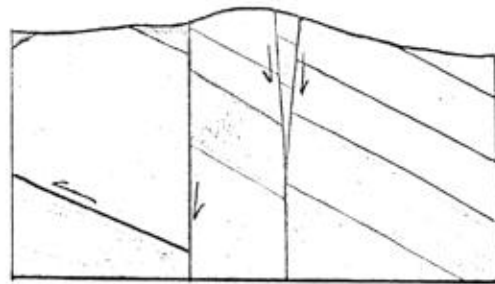
ENLARGEMENT OF ABOVE TO SHOW MANNER OF FORMATION OF THE "SLIVER" OF WALLACE CREEK
