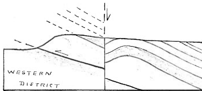
SECTION ALONG INTERNATIONAL BOUNDARY LINE
