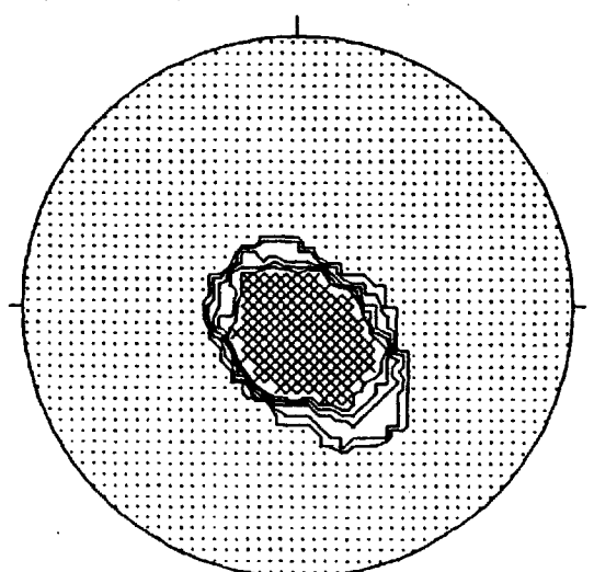
CONTOURED AT 1 2 3 + 5 POINTS PER 2.8 % AREA
