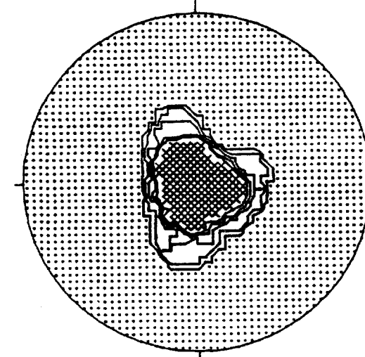
CONTOURED AT 1 2 3 + 5 POINTS PER 3.3 % AREA
