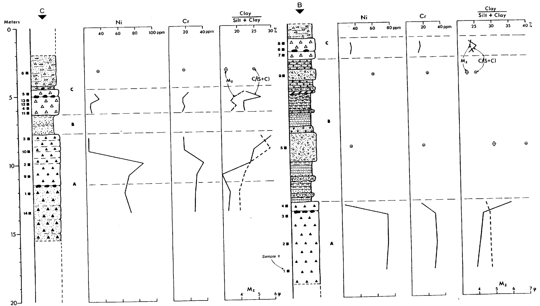
Figure 4-4 : Vertical variations of Ni and Cr contents in the silt-clay fraction (<0.063 mm) of tills and diamictos of the Norbestos section (subsections B and C). Variations of mean grain size ( M_z ) and of clay content of the silt-clay fraction are also shown. (See legend in Figure 4-12)
