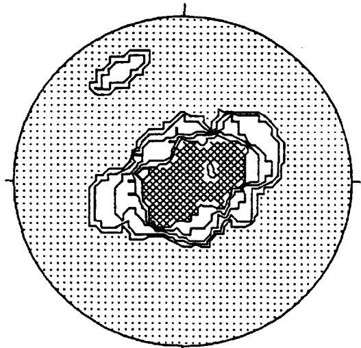
CONTOURED AT 1 2 3 4 5 POINTS PER 5.0 % AREA
