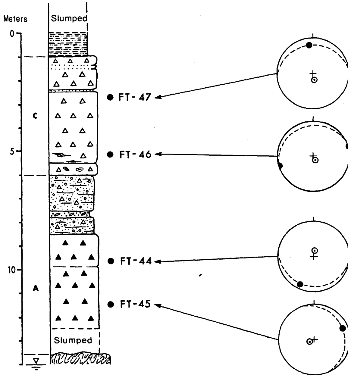
Figure 4-6 : Till clast fabrics from the Rivière des Rosiers section. (See legend in Figure 4-12)
