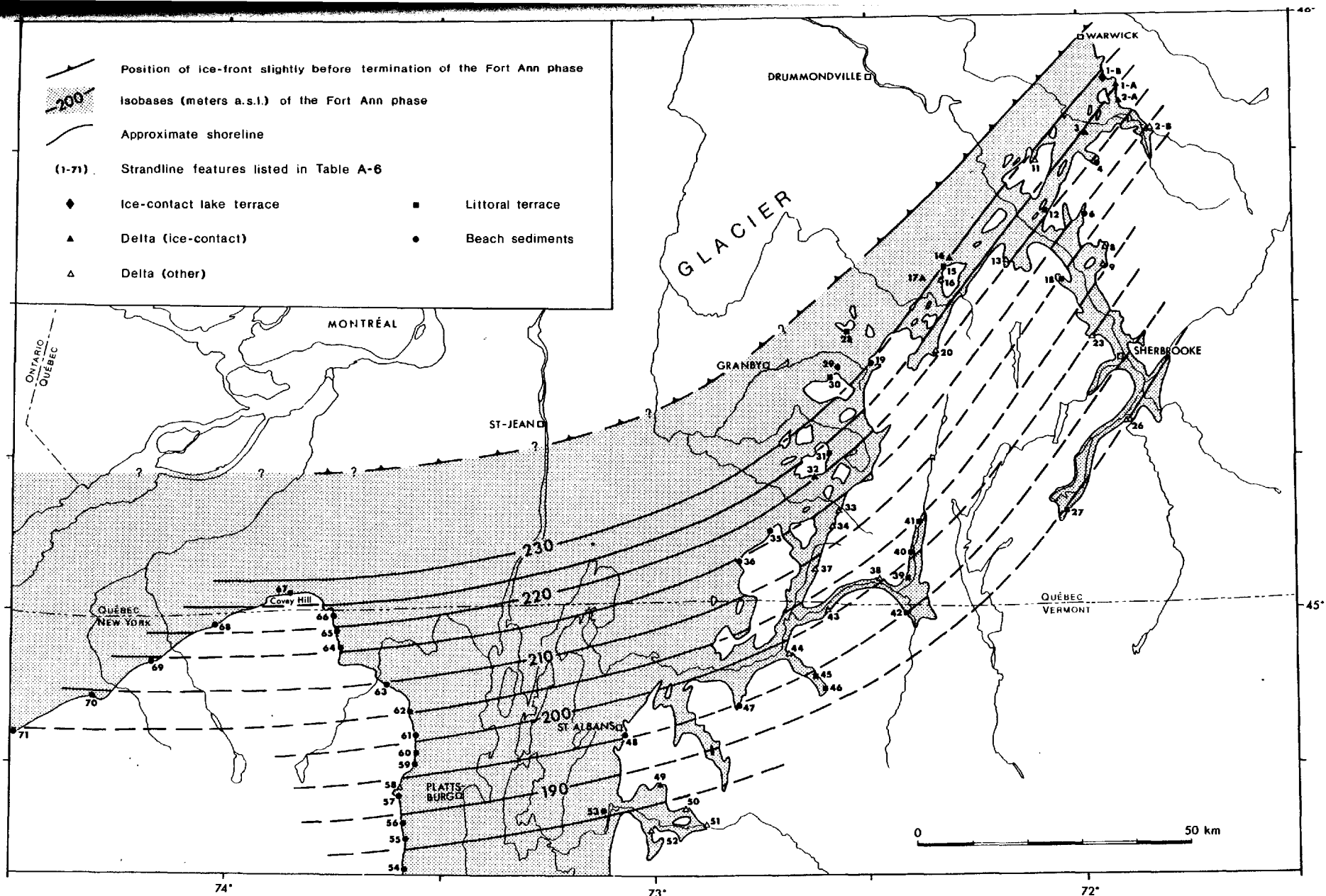
Figure 5-13 : Fort Ann phase of Glacial Lake Vermont in southern Québec and adjacent United States. Isobases on the former water-plane indicate an average geoidal flexure of \sim 1 m/km. Lake level fell when low terrains northeast of Warwick became ice-free.
