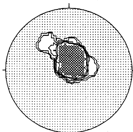
CONTOURED AT 1 2 3 + 5 POINTS PER 2.9 % AREA
