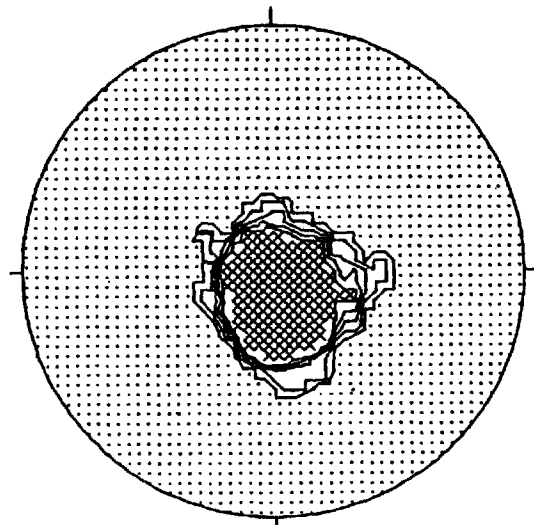
CONTOURED AT 1 2 3 + 5 POINTS PER 3.2 % AREA
