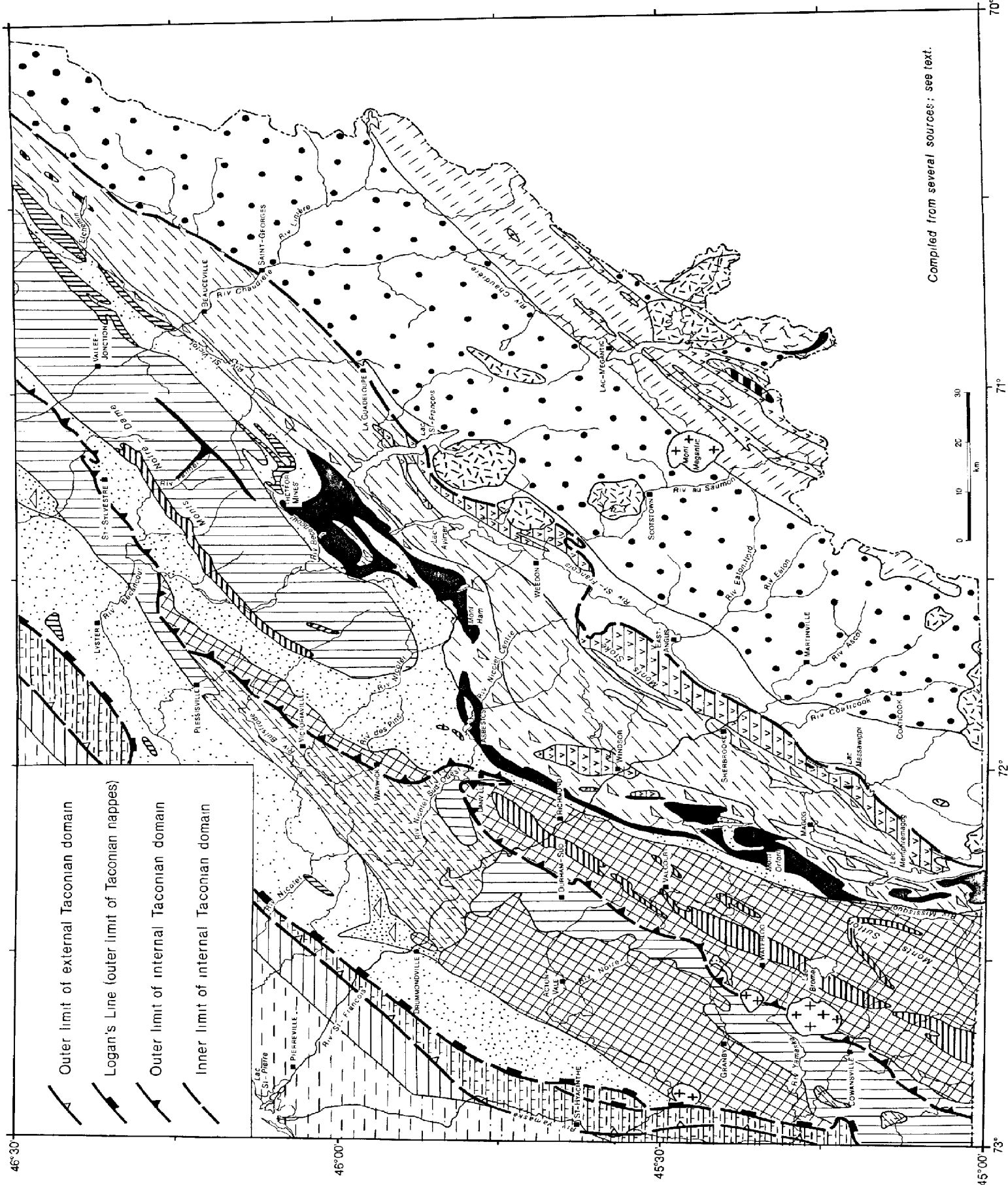
Figure 2-1: Generalized bedrock geology, southeastern Québec.
