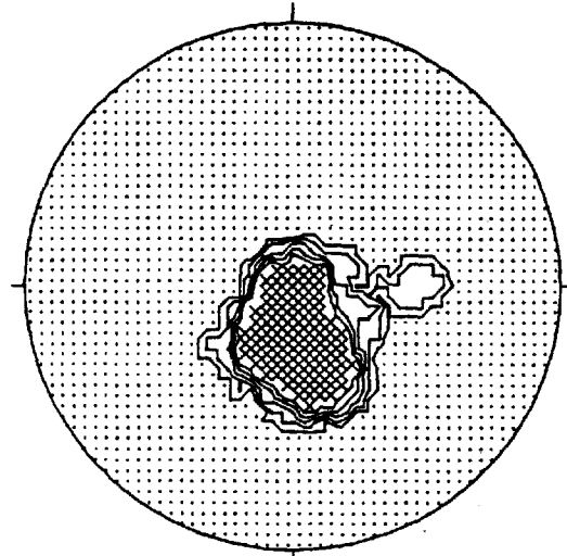
CONTOURED AT 1 2 3 4 5 POINTS PER 2.2 % AREA
