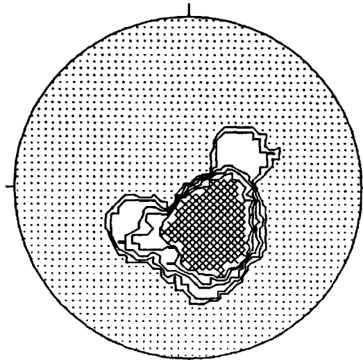
CONTOURED AT 1 2 3 + 5 POINTS PER 3.1 % AREA
