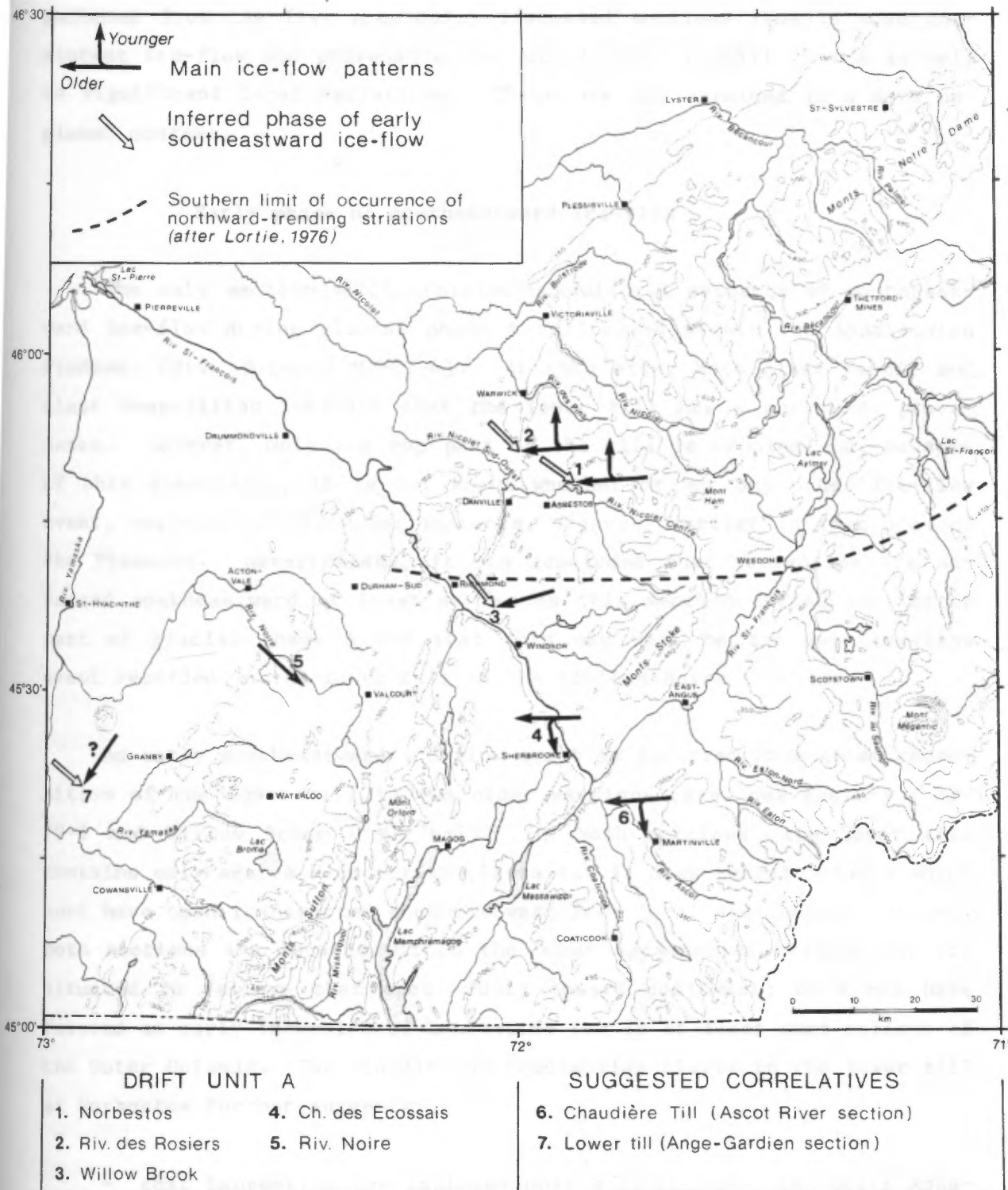
Figure 4-11: Ice-flow patterns and sequences for drift unit A and its suggested correlatives. The Ascot River (#6) and Ange-Gardien (#7) sections will be discussed in Chapter 6.
