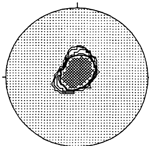
CONTOURED AT 1 2 3 + 5 POINTS PER 2.9 % AREA
