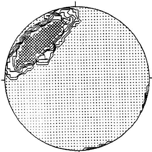
CONTOURED AT 1 2 3 + 5 POINTS PER 2.5 % AREA
