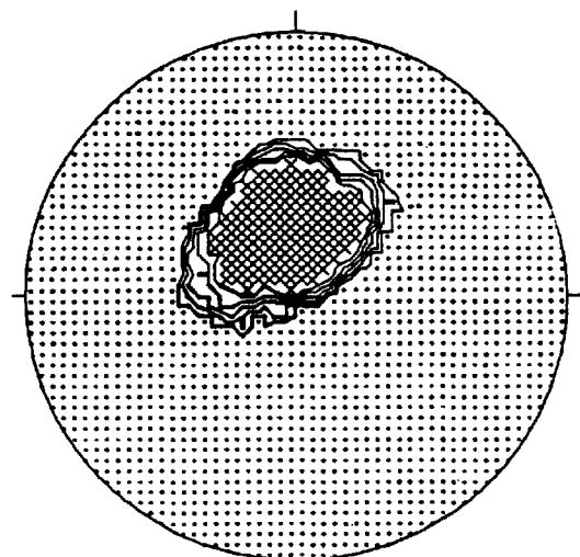
CONTOURED AT 1 2 3 4 5 POINTS PER 2.9 % AREA
