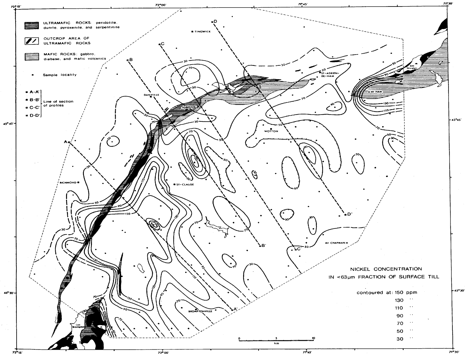
Figure 4-21: The Asbestos ultramafic dispersal train, as recorded by contour lines of Ni concentration in the silt-clay fraction ( < 0.063 mm) of surface till. Bedrock outcrop patterns are after Lamarche (1973), St-Julien (1970) and Hébert (1982). Also shown are the locations of Ni content / topographic profiles depicted in Figure 4-22.
