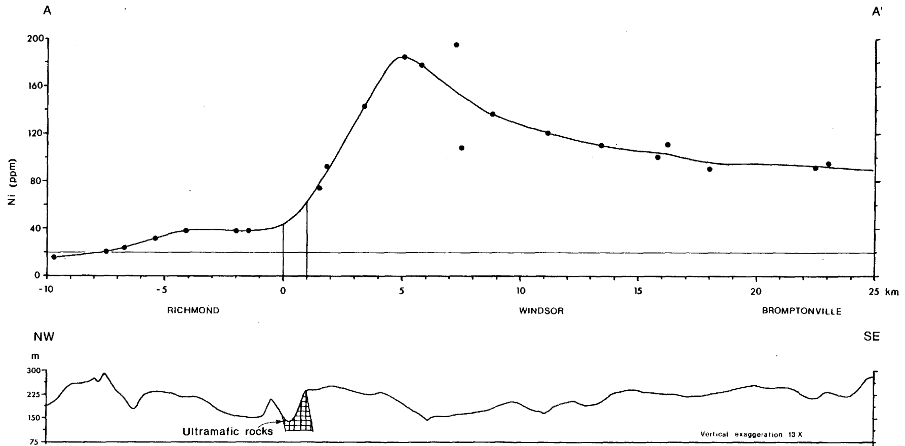
Figure 4-22 A : Topography and Ni concentration in the silt-clay fraction of surface till along profile A-A'. This profile is characteristic of Zone I of the Asbestos ultramafic dispersal train.
