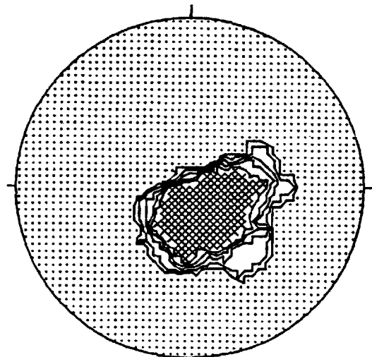
CONTOURED AT 1 2 3 + 5 POINTS PER 3.0 ° AREA
