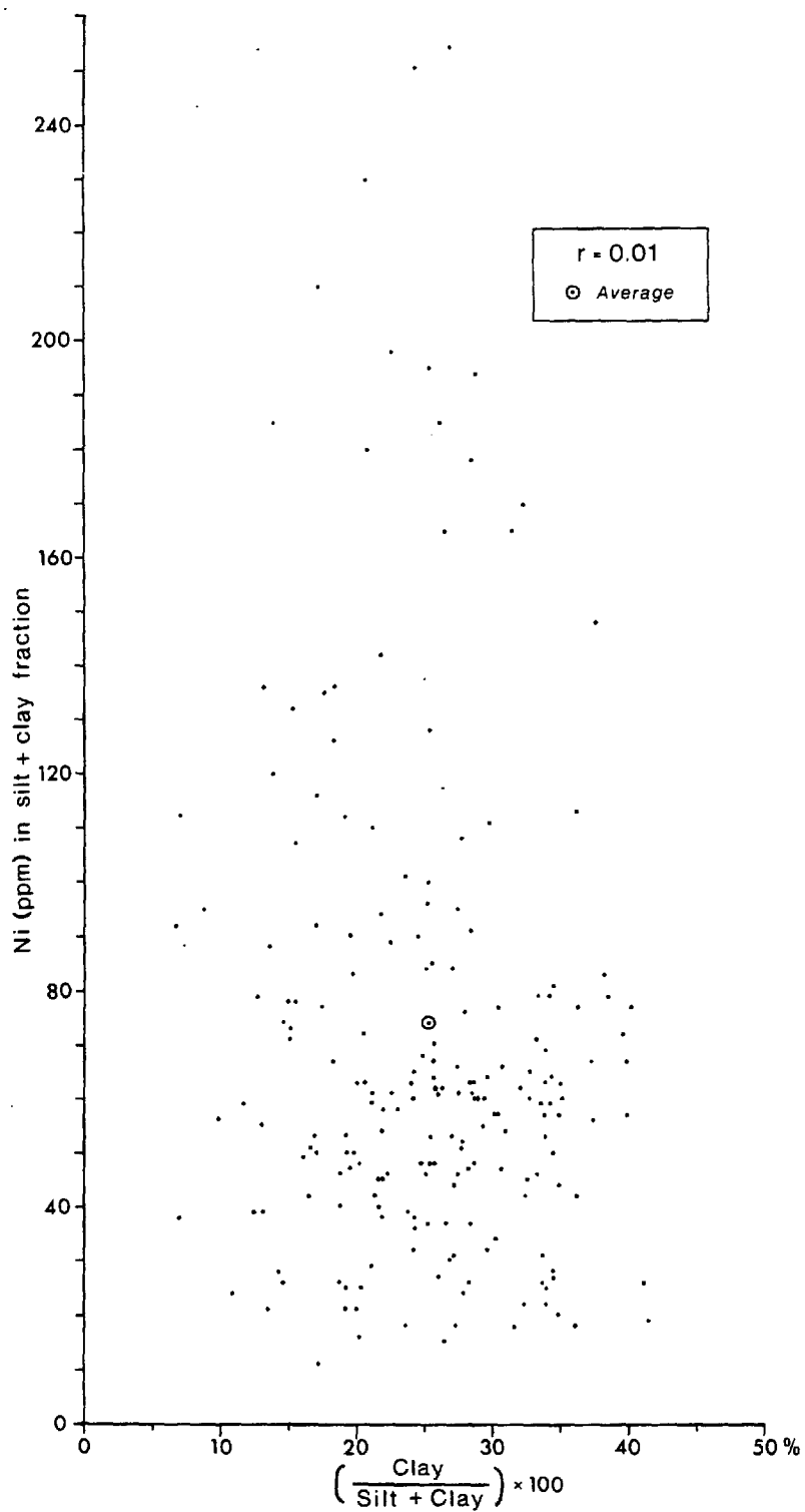
Figure 3-2 : Scatter diagram of Ni content versus clay content in the silt-clay fraction (<0.063 mm) of surface till samples. Only two of 204 samples have a Ni content (450 and 275 ppm) beyond the range of the diagram (see Table A-3 : samples #80-155 and #80-156).
