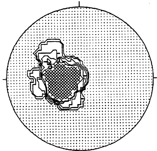
CONTOURED AT 1 2 3 + 5 POINTS PER 3.4 % AREA
