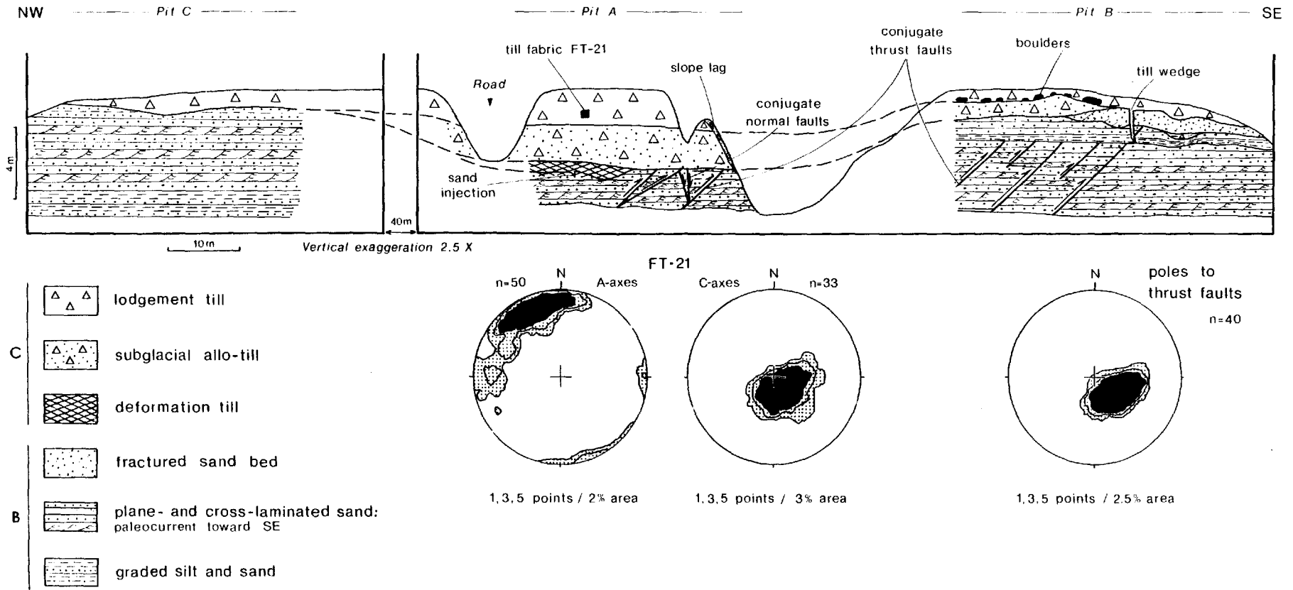
Figure 4-13 : Stratigraphy and lithofacies at the Wotton section (MP-79-5), showing lateral relationships of lithofacies units and glacitectonic deformations. Contoured stereograms of poles to thrusts faults and of a till clast fabric are also shown.
