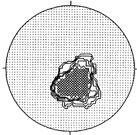
CONTOURED AT 1 2 3 + 5 POINTS PER 2.9 % AREA
