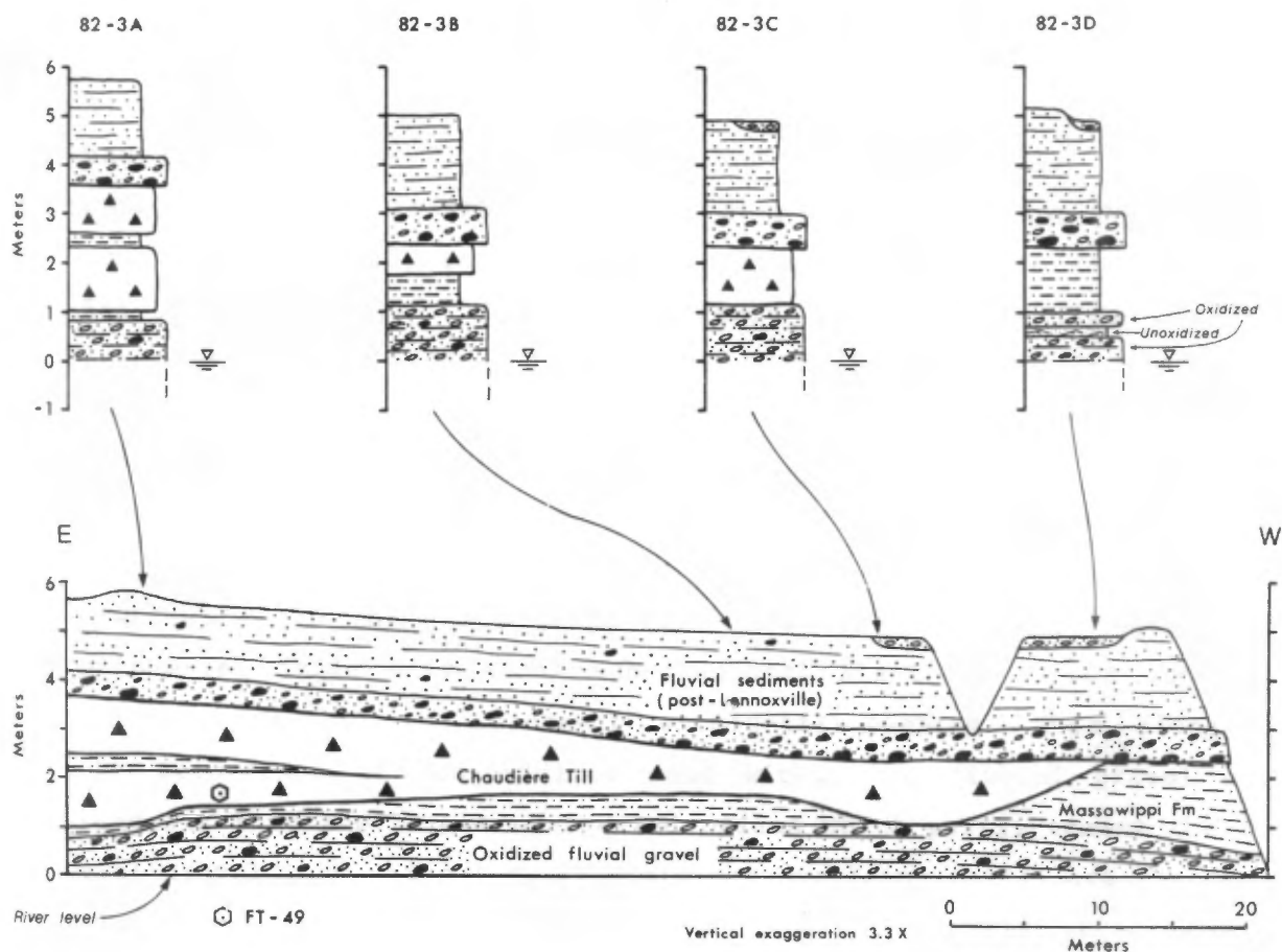
Figure 6-3 : Lateral relationships of units exposed in the second Ascot River section (MP-82-3). Notice the absence of Johnville Till between the oxidized fluvial gravel and the Massawippi Formation. Oxidation of the lowermost fluvial gravel unit is interpreted as the result of modern groundwater aeration (see text).
