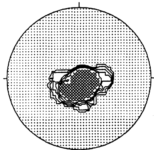
CONTOURED AT 1 2 3 + 5 POINTS PER 2.6 % AREA
