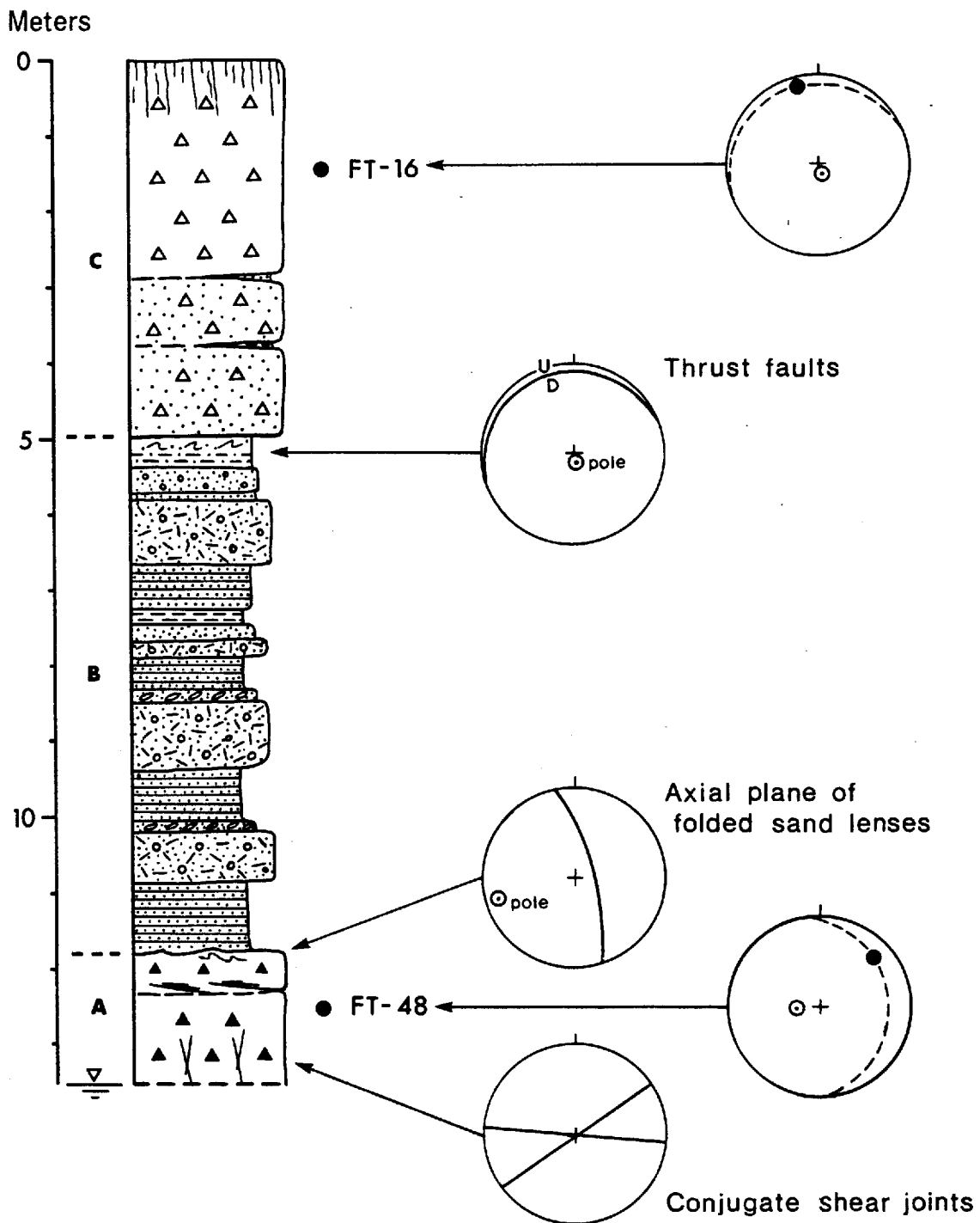
Figure 4-7 : Stratigraphic log, till clast fabrics and attitudes of glactectonic deformations, Willow Brook section (MP-76-1). (See legend in Figure 4-12)
