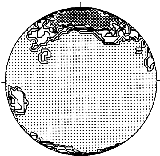
CONTOURED AT 1 2 3 4 5 POINTS PER 2.0 % AREA
