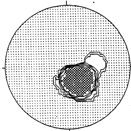
CONTOURED AT 1 2 3 + 5 POINTS PER 4.0 % AREA
