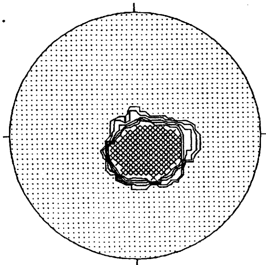
CONTOURED AT 1 2 3 + 5 POINTS PER 2.6 % AREA
