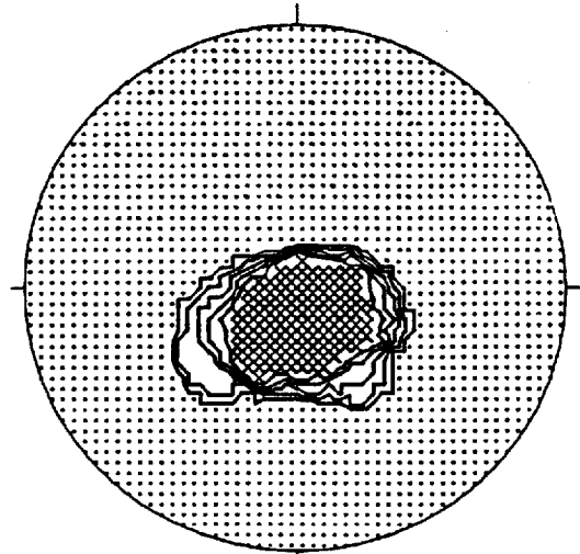
CONTOURED AT 1 2 3 4 5 POINTS PER 3.4 % AREA
