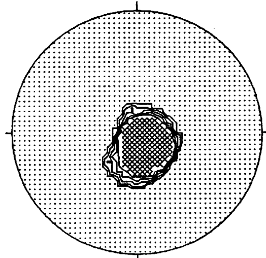
CONTOURED AT 1 2 3 4 5 POINTS PER 2.4 % AREA
