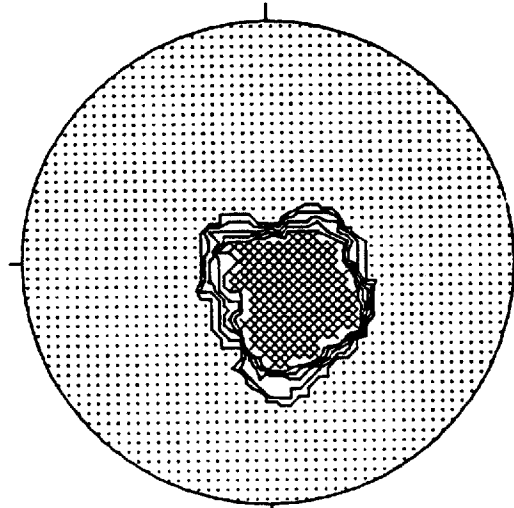
CONTOURED AT 1 2 3 4 5 POINTS PER 2.1 % AREA
