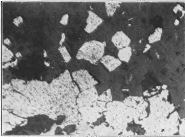
Polished section of specimen from north margin of No. 6 ore-body. \times 66 . Pyrite, white; quartz, dark grey; chlorite, black.—The pyrite is fractured and some non metallics, later than the pyrite, fill the fractures.
