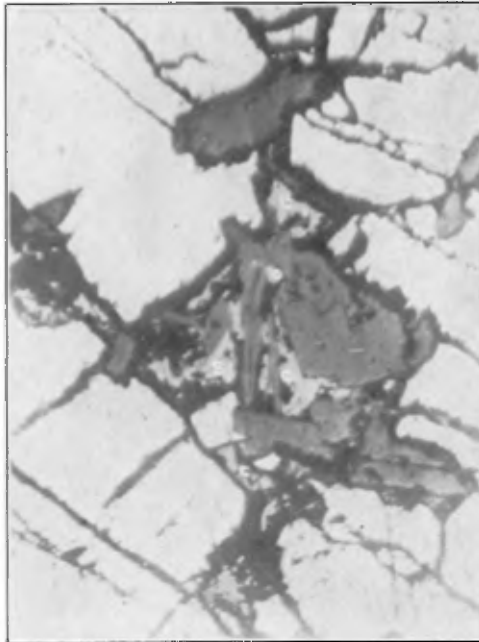
Polished specimen of ore from point south of north margin of No. 6 ore-body. \times 66 . (C) chalcopyrite; (S) sphalerite; (white) pyrite; (dark grey) chlorite.
