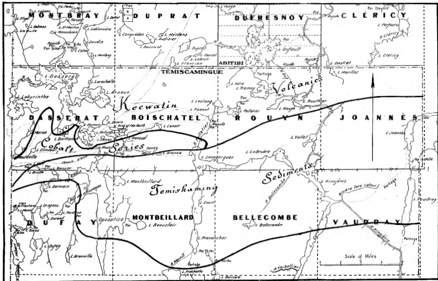
Sketch map showing outlines of geological formations in new gold fields. The interesting belt is parallel to contact line between Temiscaming sediments and Keewatin Volcanics, from 1\frac{1}{2} miles south of this line to 6 miles north of it.
