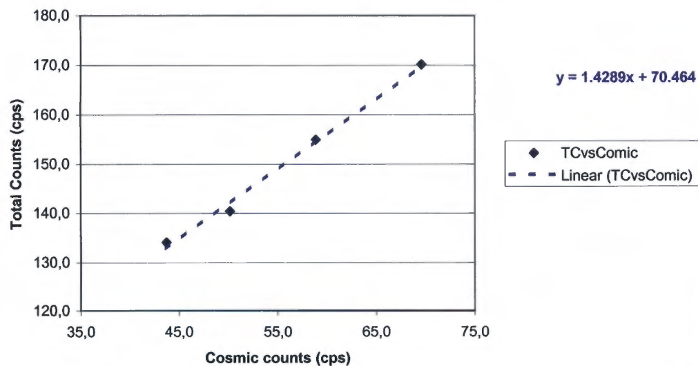
Total Counts vs Cosmic counts
