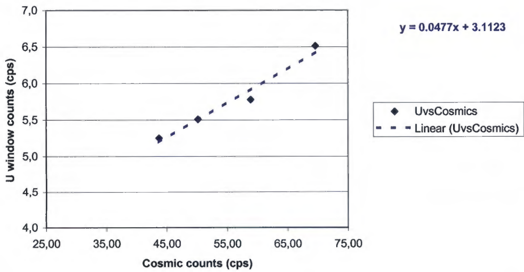
U window counts vs Cosmic counts
