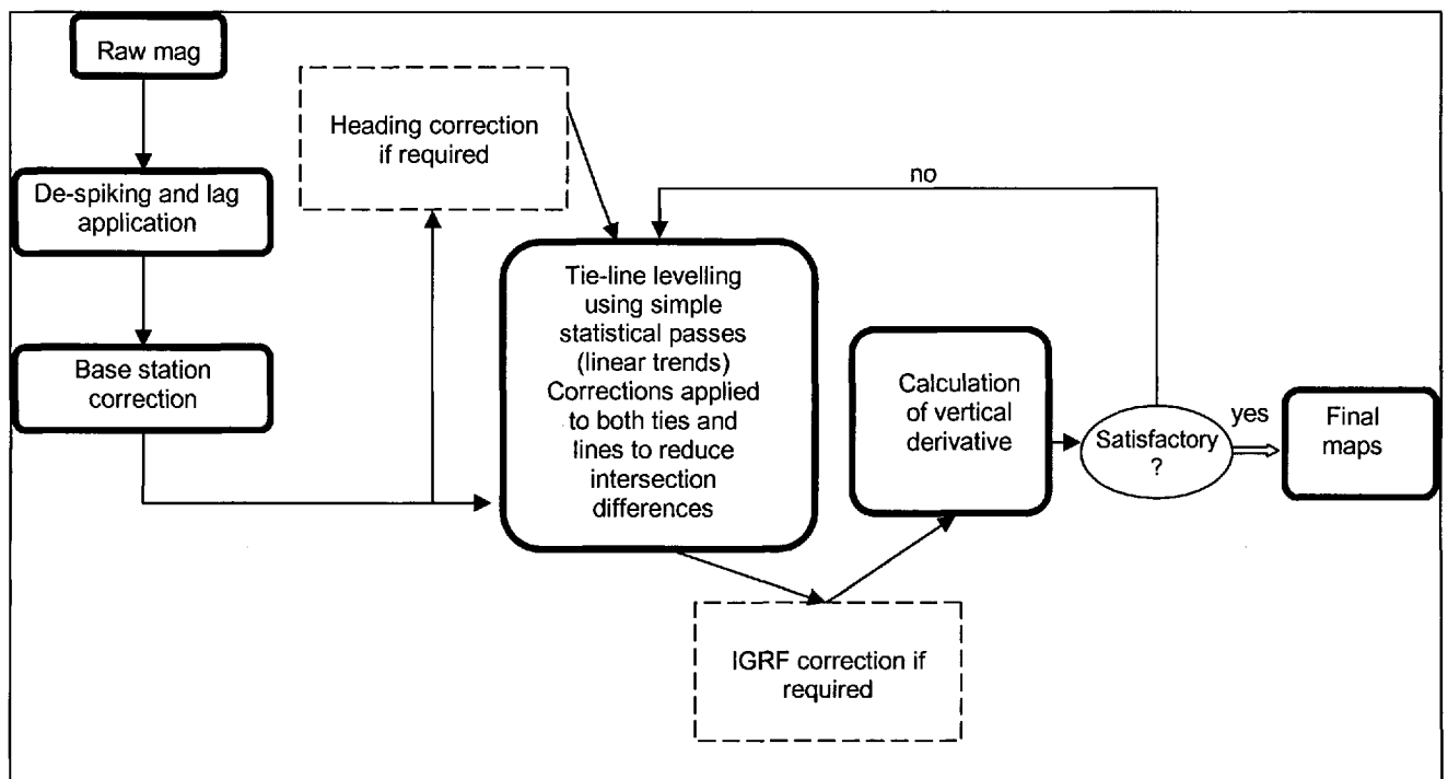
Figure 4 – Standard magnetic data processing flow
