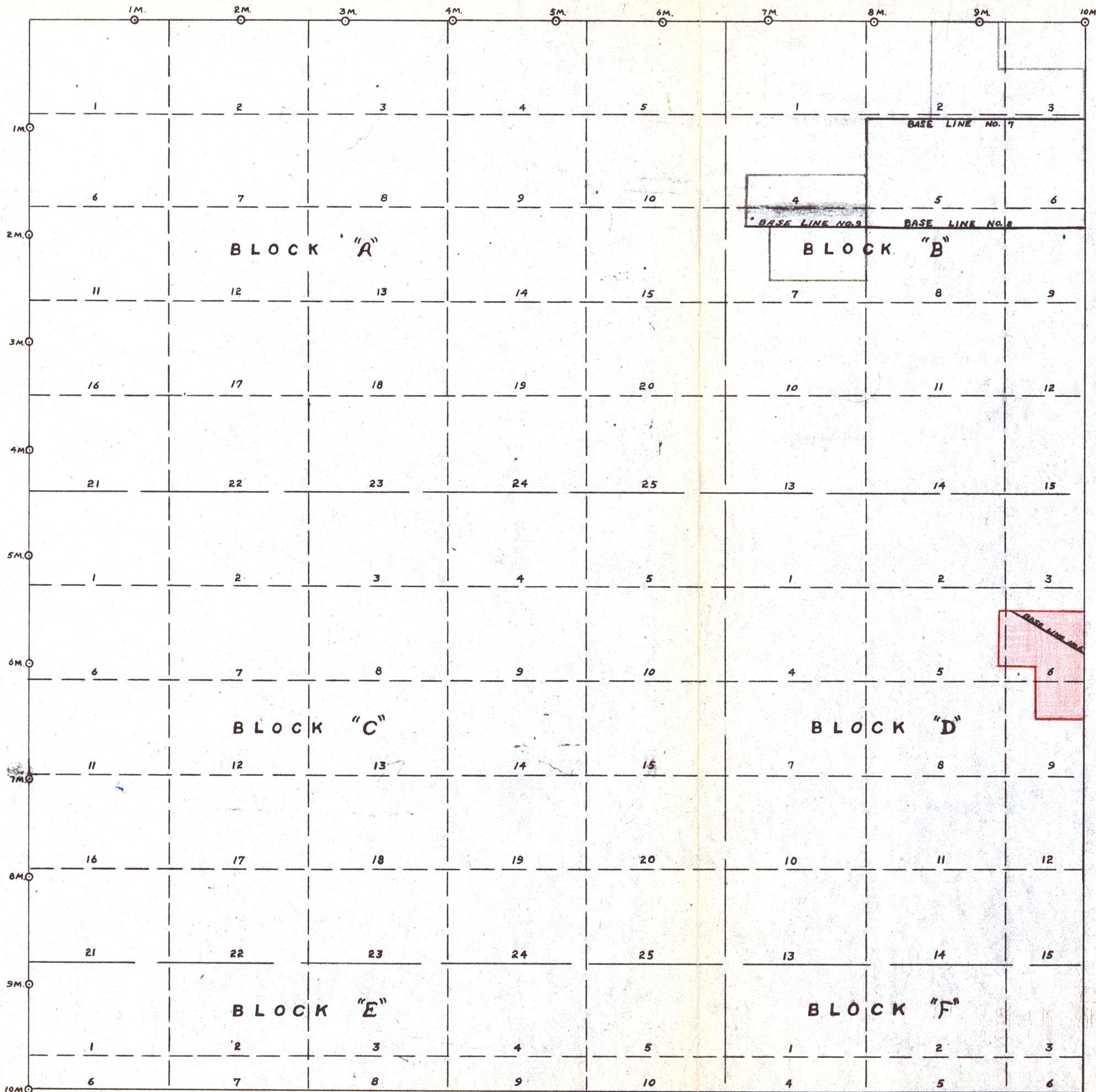
QUEBEC TOWNSHIP LAYOUT PLAN FOR 1000 AND 200 SCALE MAP SHEETS. SCALE:- 1" = 1 MILE.
